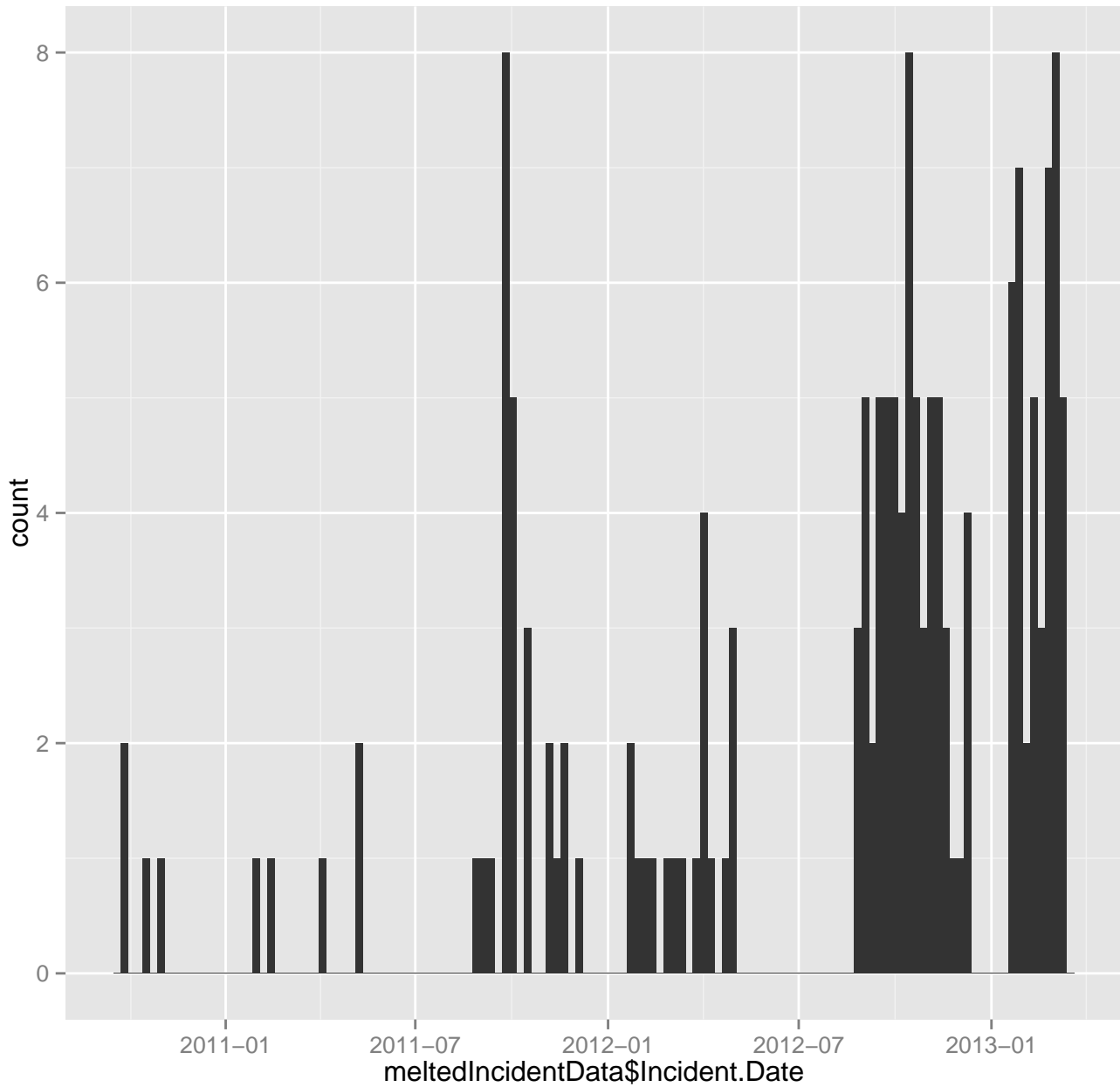
Binwidth 7
