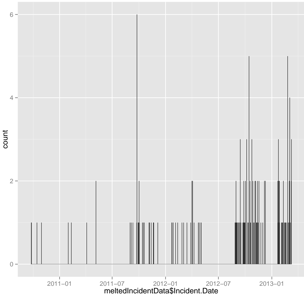
Binwidth 1
