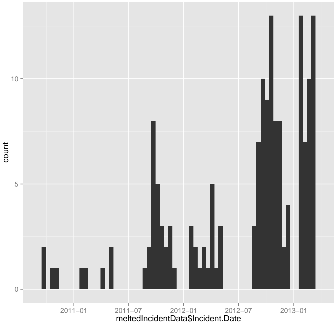
Binwidth 14
